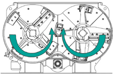
Synchronised and alternating mixing axis rotation
