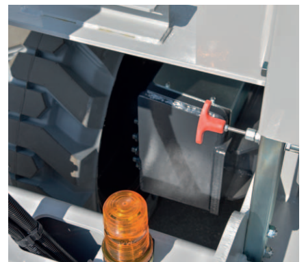
Platform manual emergency descent control
