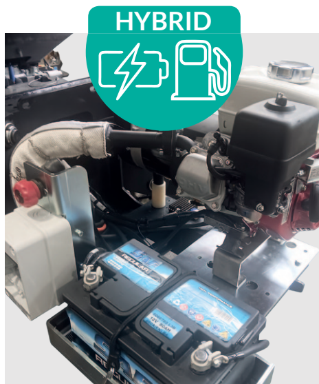
Petrol generator and lithium battery group (hybrid version).
